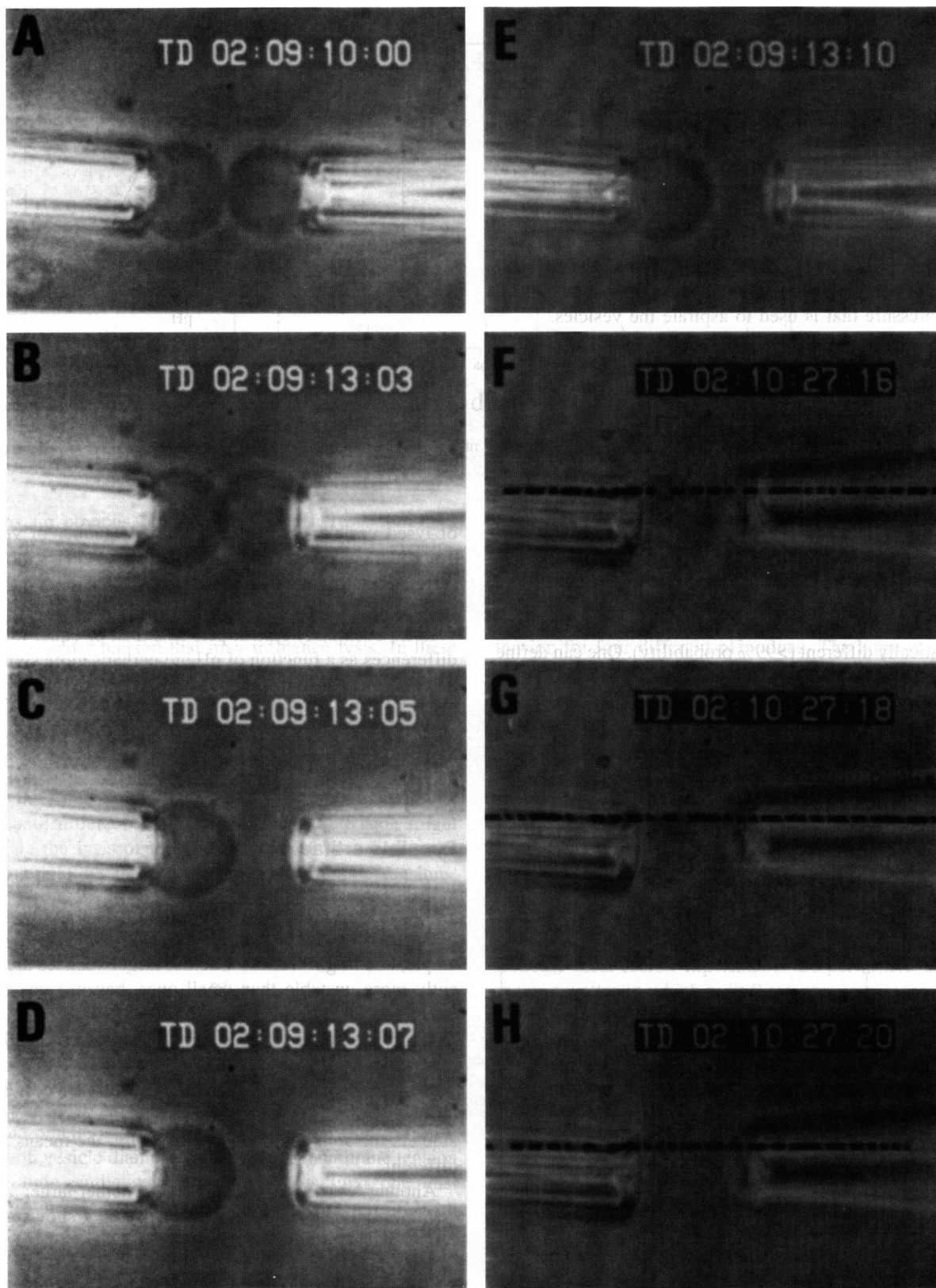
FIGURE 4 Video time sequence showing lysis induced by peptide X31. Numbers at the top of each frame indicate the time code for that frame (h: min:s:frames). Peptide X31 at 10 \mu M and pH 5 was injected at time 2:09:10:00. The dashed line seen in F, G, and H is an artifact produced by our VCR. (A) Vesicles in contact at the time of injection. (B) Right vesicle begins to lyse. (C–E) Right vesicle shrinks and disappears, characteristic of lysis. (F) Left vesicle begins to lyse. (G–H) Left vesicle shrinks and disappears..
